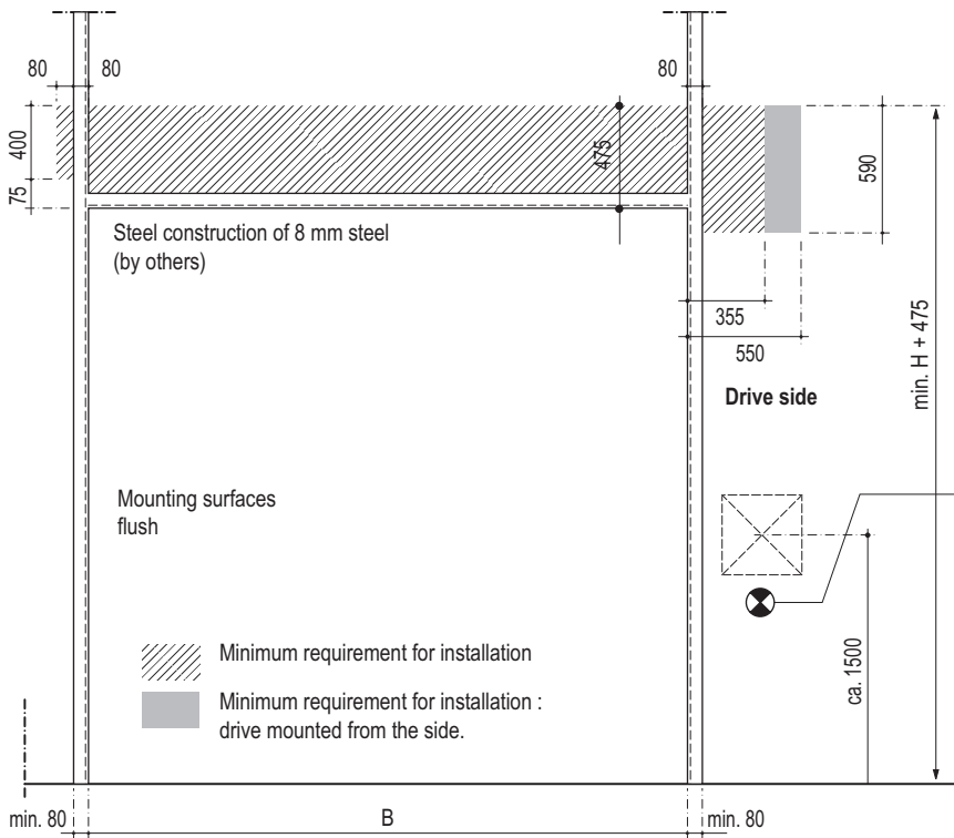
Section A
