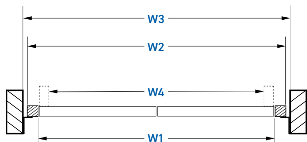
Fitting within the opening
