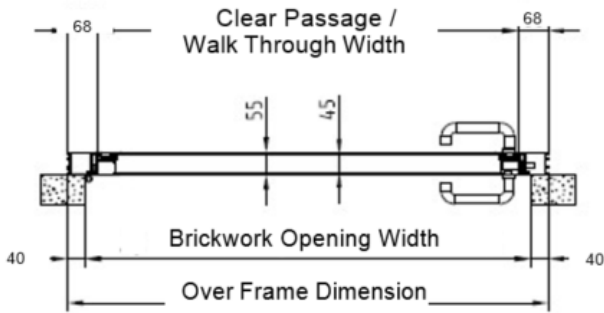
Horizontal Cut (Installation behind the opening)
